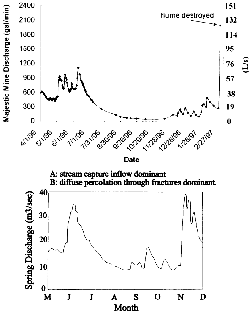
Figure 8 Comparison of the Majestic Mine hydrograph (upper Figure) with a karst spring (bottom). Karst hydrograph after Brogli (1980)
