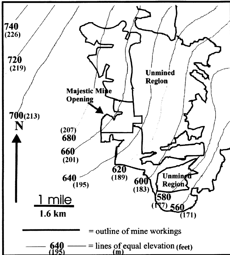
Figure 3. Structure contour map of the Middle Kittanning (No. 6) Coal (from Ohio Geological Survey non dated, 15-minute Athens Quadrangle).
